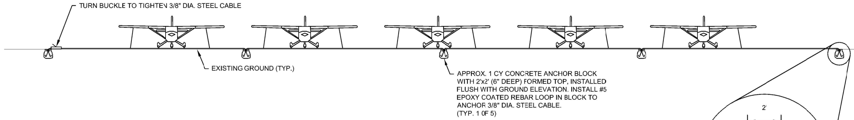
PROFILE VIEW NOT TO SCALE
