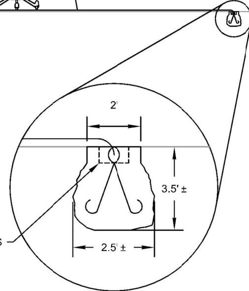
BLOCK DETAIL NOT TO SCALE
