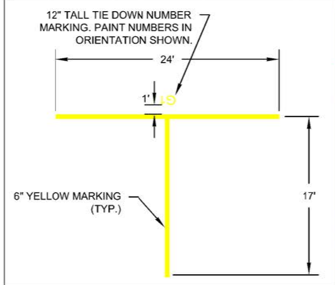
TIE DOWN MARKING DETAIL NTS
