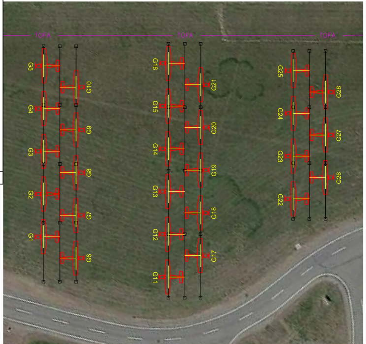
TIE DOWN MARKING DETAIL NTS
